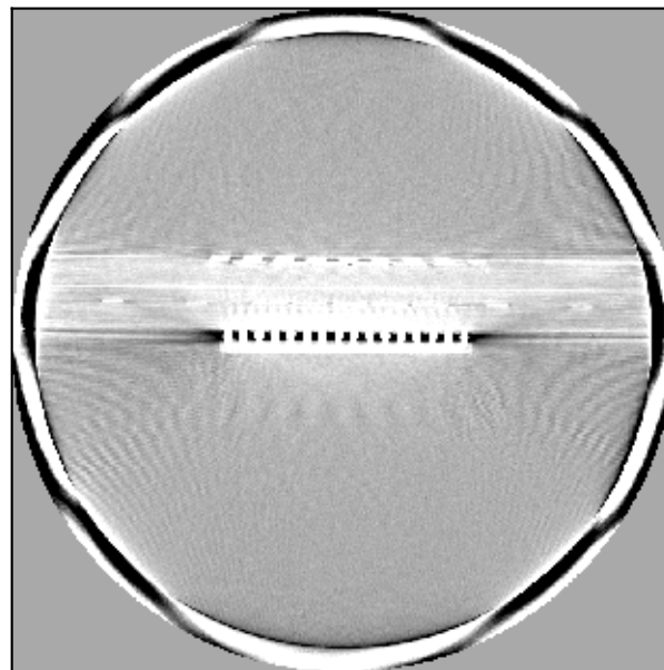
BGA --- damped
