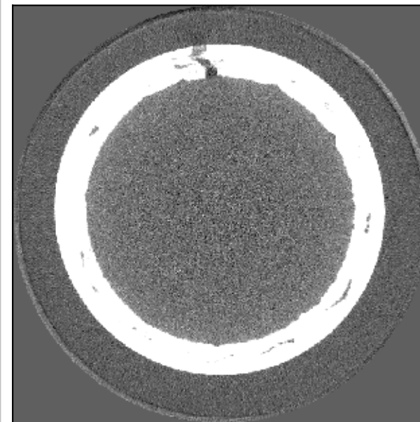
SiC --- undamped
